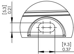
VIEW A
